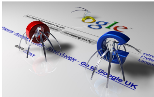
Web harvesting
